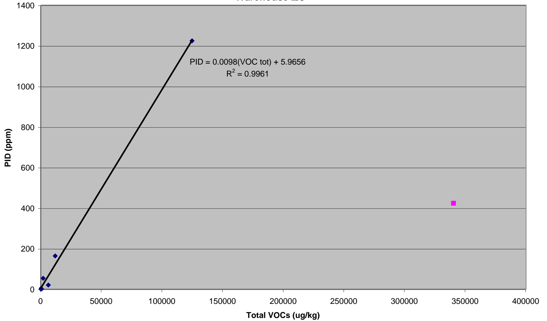
Figure 3 PID vs Total VOCs Warehouse 2/3
